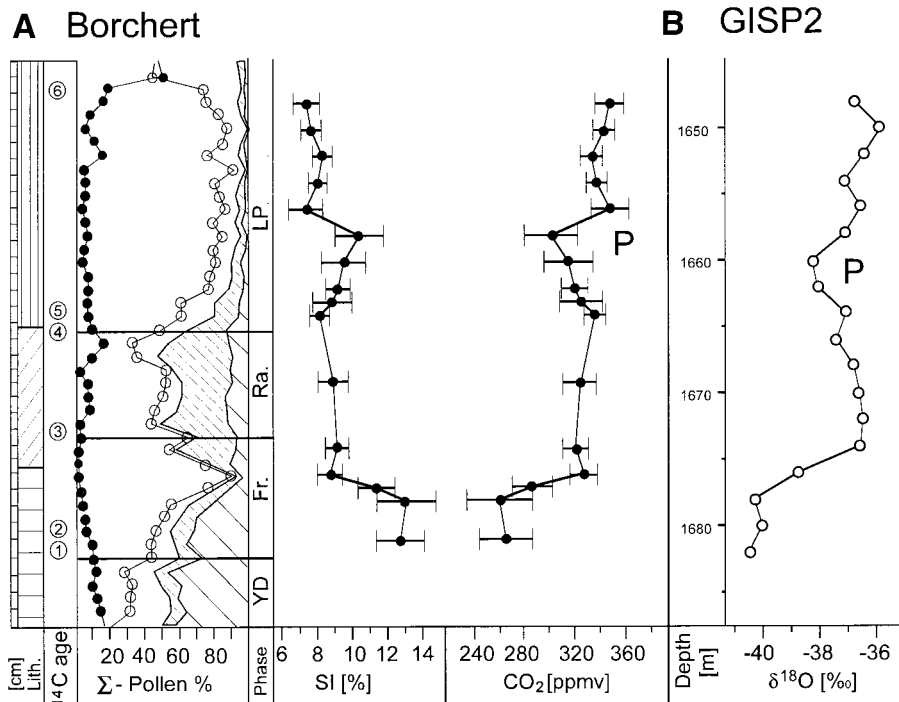
Fig. 1. (A) Mean SI values (±1σ) for B. pendula and B. pubescens from the early Holocene part of the Borchert section (Netherlands; 52.23°N, 7.00°E) and reconstructed CO 2 concentrations. The scale of the section is in centimeters. Three lithological (Lith.) units can be recognized (18): a basal gyttja (=), succeeded by Drepanocladus peat (//), which is subsequently overlain by Sphagnum peat (||). Six conventional 14 C dates (in years before the present) are available (indicated by circled numbers): 1, 10,070 ± 90; 2, 9930 ± 45; 3, 9685 ± 90; 4, 9770 ± 90; 5, 9730 ± 50; and 6, 9380 ± 80. Summary pollen diagram includes arboreal pollen (white area) with Pinus (●) and with Betula (○) and nonarboreal pollen with Gramineae (\\) and with Cyperaceae, upland herbs, and Ericales (\\). Regional climatic phases after (18): YD, Younger Dryas; Fr., Friesland phase; Ra., Rammelbeek phase; and LP, Late Preboreal. For analytical method, see (13). Quantification of CO 2 concentrations according to the rate of historical CO 2 responsiveness of European tree birches (Fig. 2). P indicates the reconstructed position of the Preboreal Oscillation. (B) δ 18 O profile for the Younger Dryas–Holocene transition in the Greenland GISP2 ice core, after (20); P denotes the δ 18 O-inferred cooling of the Preboreal Oscillation, starting at ~11,300 calendar years before the present (3).
